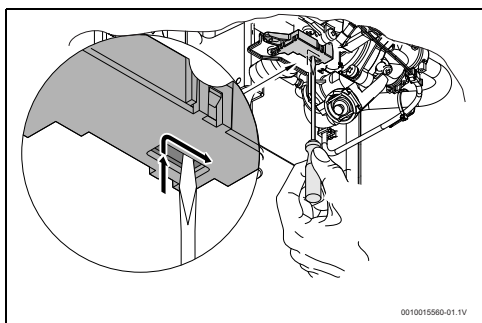
Fig. 24 Rearme do micro-interruptor
